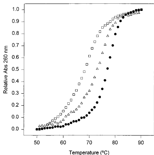
Figure 2. Thermal denaturation curves for control duplex 7-12 (●), Os II -containing duplex 9-12 (△), and a single-mismatch duplex 7-14 (□) determined in 0.01 M sodium phosphate buffer pH 7, 0.1 M NaCl. 8
